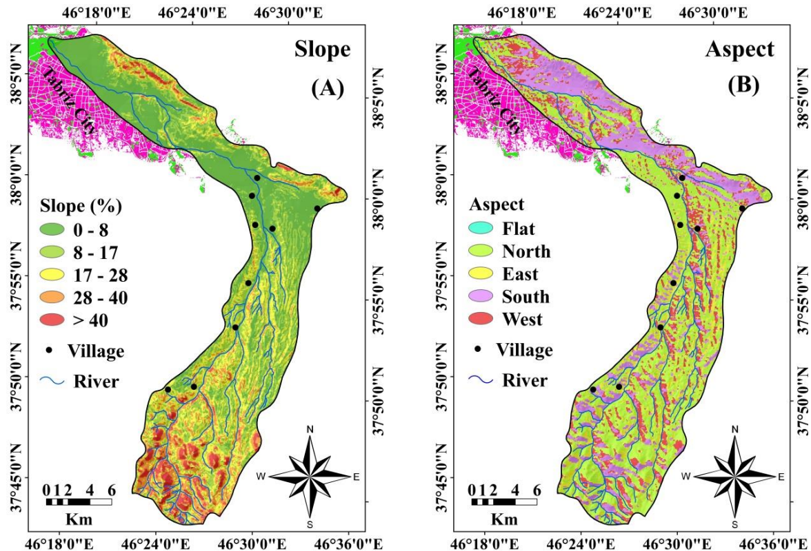
Figure 4. Slope and Aspect map
