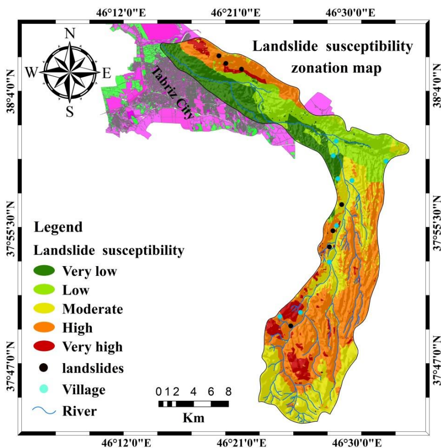
Figure 7. Landslide susceptibility zonation map of Mehran Roud basin based on the ANP model
